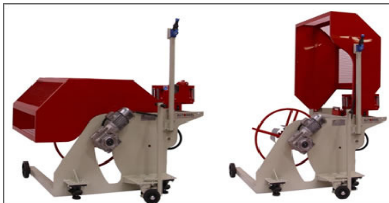
An electrically interlocked guard is now standard on SCW machines
